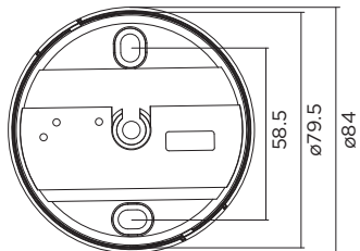
Ceiling base dimensions
